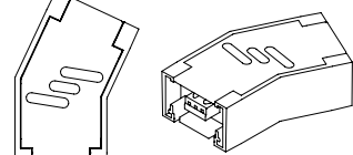
CONECTOR 155°
